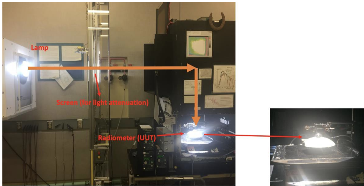
Figure 1: NREL's X25 solar simulator setup to measure the nonlinearity of pyranometer.
