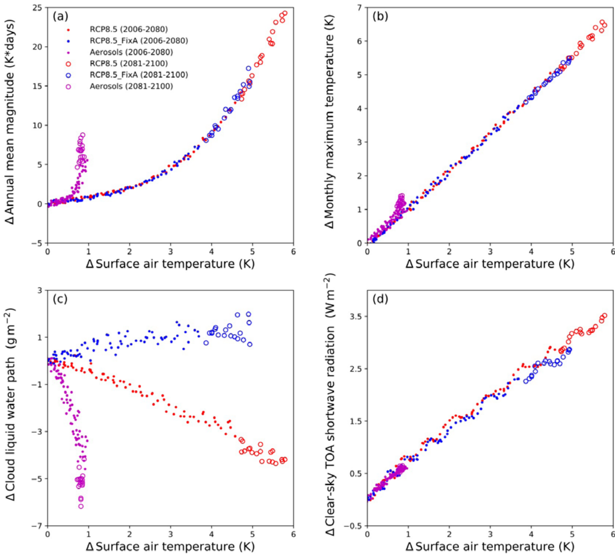
Figure 1. Scatter-plots of changes (ensemble mean of annual mean) in land area-weighted mean heatwave magnitude ( K \cdot \text{days} ) against global land mean surface temperature change. Also shown are changes in the annual mean of global area-weighted mean (b) monthly maximum temperature ( TX , K ), (c) cloud liquid water path ( g \text{ m}^{-2} ) and (d) total net clear-sky shortwave radiation at top-of-the-atmosphere ( W \text{ m}^{-2} ), all plotted against land area-weighted mean surface temperature change ( K ). All scatterplots are plotted separately for the period 2006–2080 (filled small dots) and 2081–2100 (large circles). The color conventions are: red for RCP8.5 (GHGs + aerosols), blue for RCP8.5_FixA (GHGs only) and magenta for aerosols, isolated by the difference RCP8.5 - RCP8.5_FixA.
