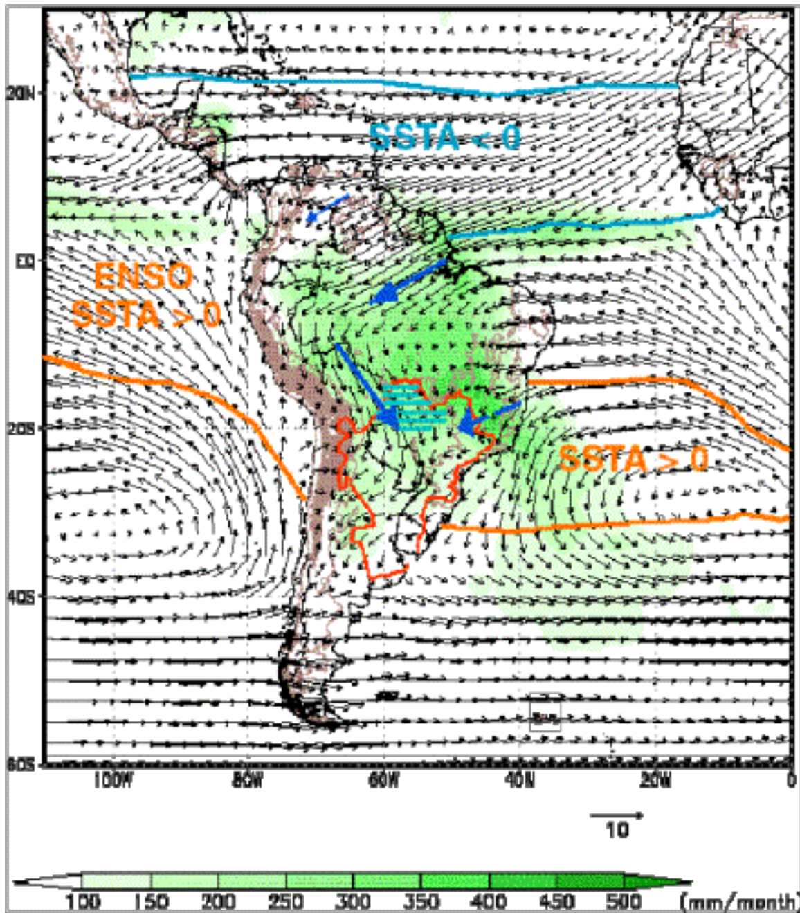
Figure 13. Links between climate variability in the Plata River Basin (area encircled by the red curve) and SST anomalies for the southern warm season (December-February). Green shading corresponds to precipitation (mm/month), black arrows to 925 hPa winds, thick blue arrows to maxima in vertically integrated moisture transport, and the blue hatched region to the Pantanal. The configuration of SST anomalies corresponds to enhanced precipitation in the basin.
