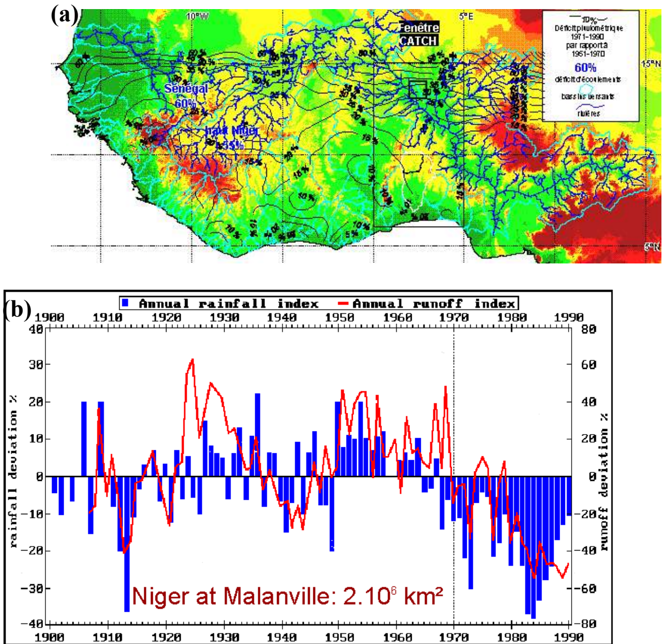
Figure 8: a) Rainfall and basin deficits (in %) for West Africa between wet period (1951-1970) and dry period (1971-1990) and b) Time series of annual rainfall deficit and annual runoff deficit for the Niger river at Malanville.
