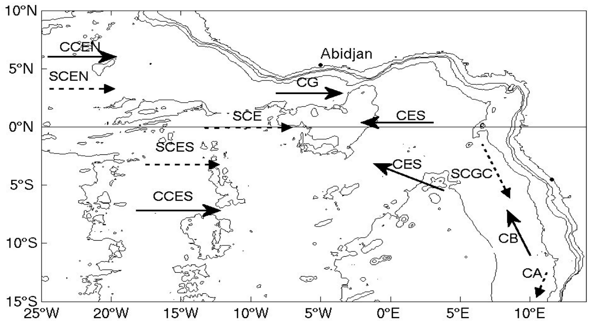
Figure 10: Mean surface and subsurface Currents in the eastern tropical Atlantic. Surface currents - full arrows- : North Equatorial CounterCurrent (CCEN) ; Guinea Current (CG) ; South Equatorial CounterCurrent (CCES) ; South Equatorial Current (CES) ; Benguela Current (CB). Subsurface currents -dashed arrows- : North Equatorial UnderCurrent (SCEN) ; Equatorial UnderCurrent (SCE) ; South Equatorial UnderCurrent (SCES) ; Gabon-Congo UnderCurrent (SCGC) ; Angola Current
