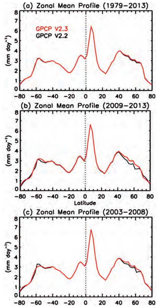
Figure 2. Zonal mean profiles of GPCP oceanic precipitation during three time periods.
